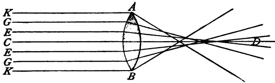
FIG. 55.—Spherical aberration.
